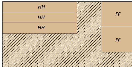
49" x 97" - 3/4" MDF
