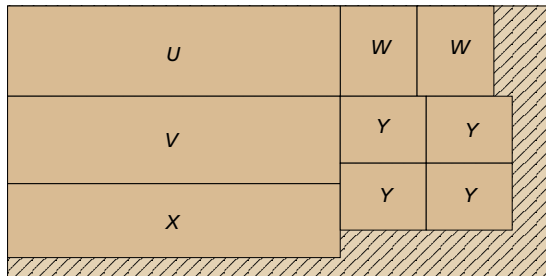
49" x 97" - 3/4" MDF
